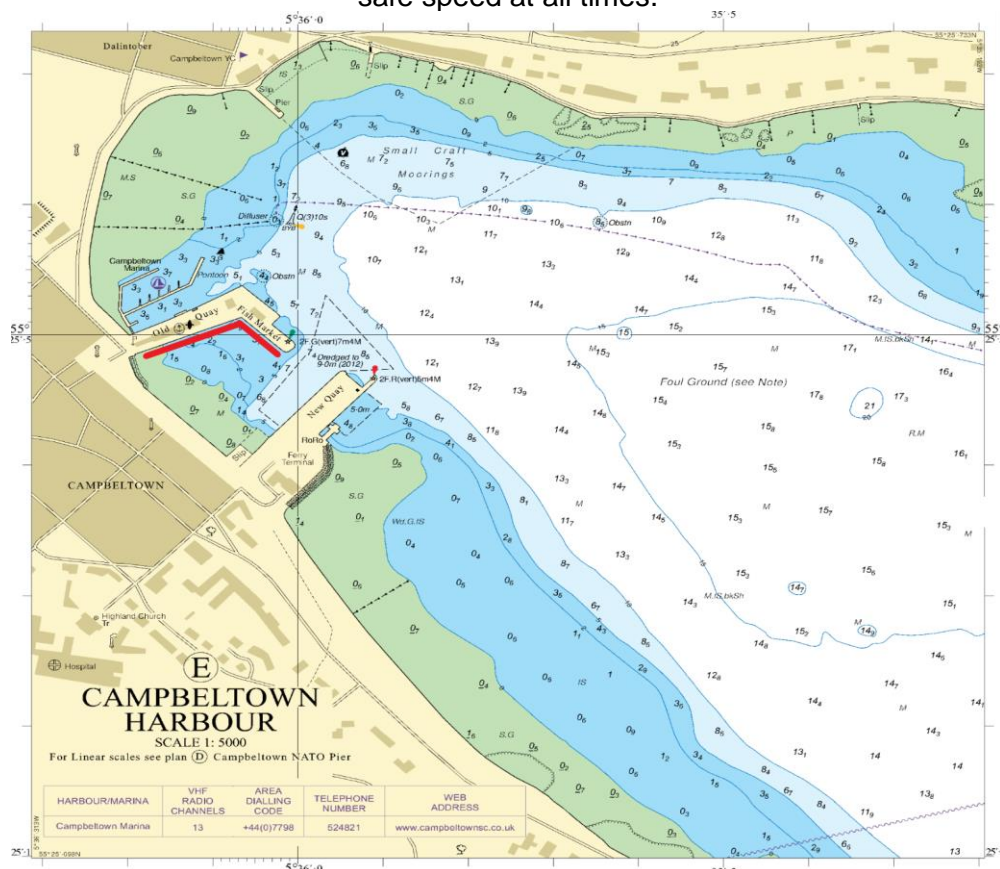
FIG: RED LINE DENOTES BERTHS AFFECTED BY DREDGING WORKS
